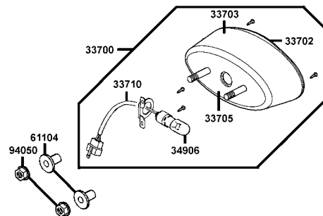
F16 Rear Light
